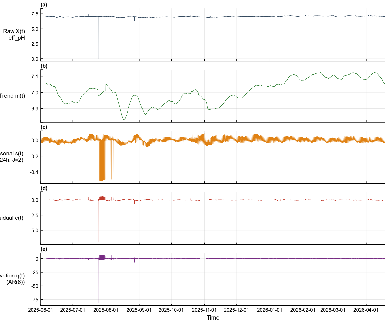
Multi-scale decomposition — eff_pH (effluent, hour) [2025-06-01~2026-04-19]
